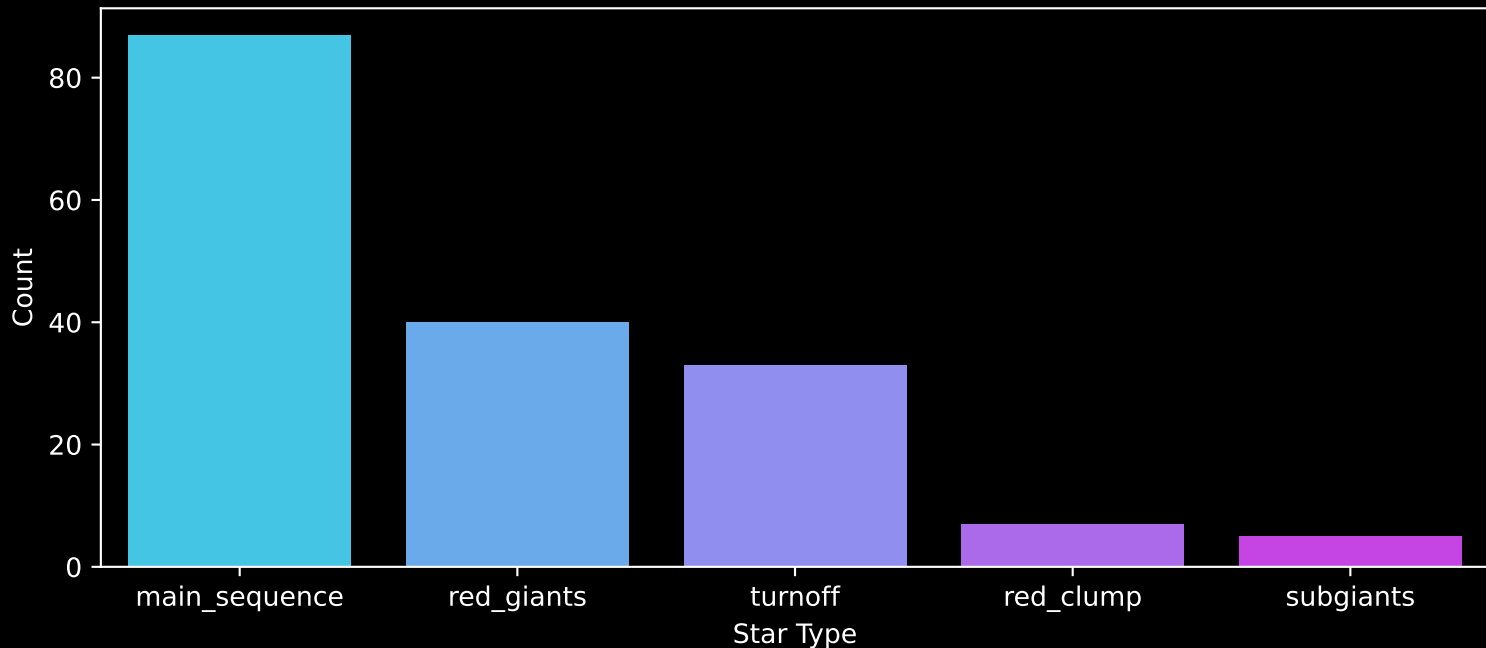
APOGEE DR17 Field: [053+33_MGA] Count plot of Star Type
