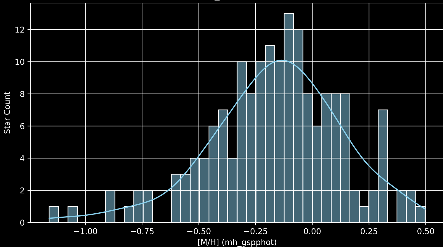
APOGEE DR17 Field: [053+33_MGA [M/H] (mh_gspphot) (n= 169)
