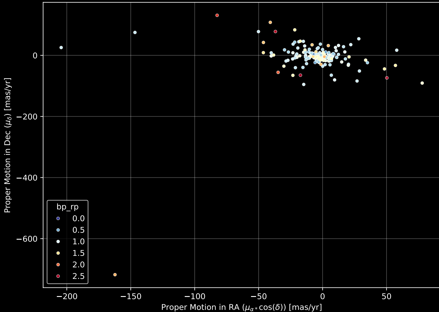
APOGEE DR17 Field: [053+33_MGA] Proper Motion Diagram (n= 172)
