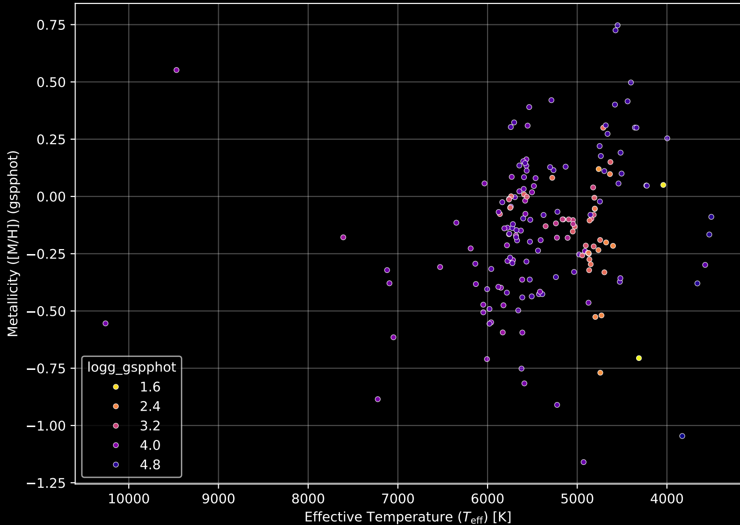
APOGEE DR17 Field: [053+33_MGA] Stellar Population Parameters (n= 172)
