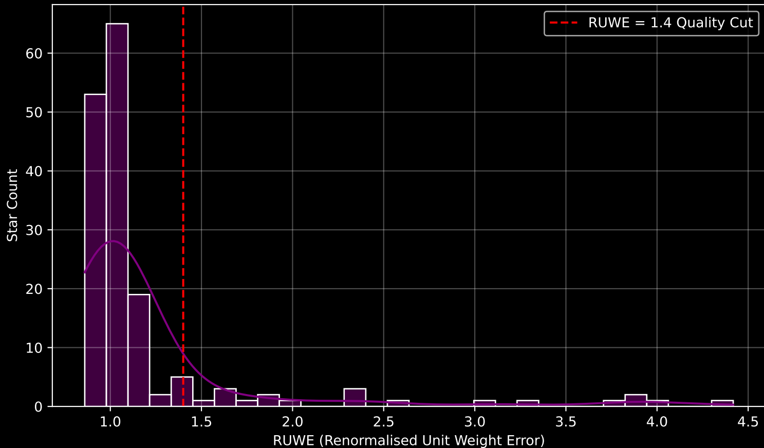
GAPOGEE DR17 Field [053+33_MGA] RUWE Distribution (n= 163)
