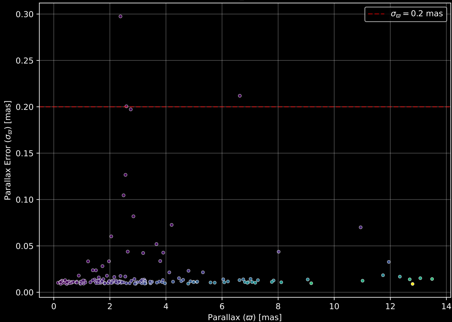
APOGEE DR17 Field: [053+33_MGA] Parallax Quality (n= 172)
